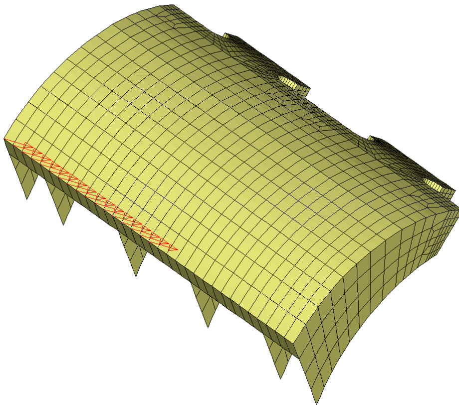
GRP Saddle structure FEM model with edge loading
